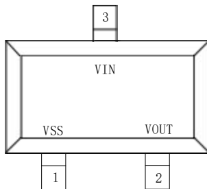
SOT23-3L/SOT23B (TOP VIEW)
